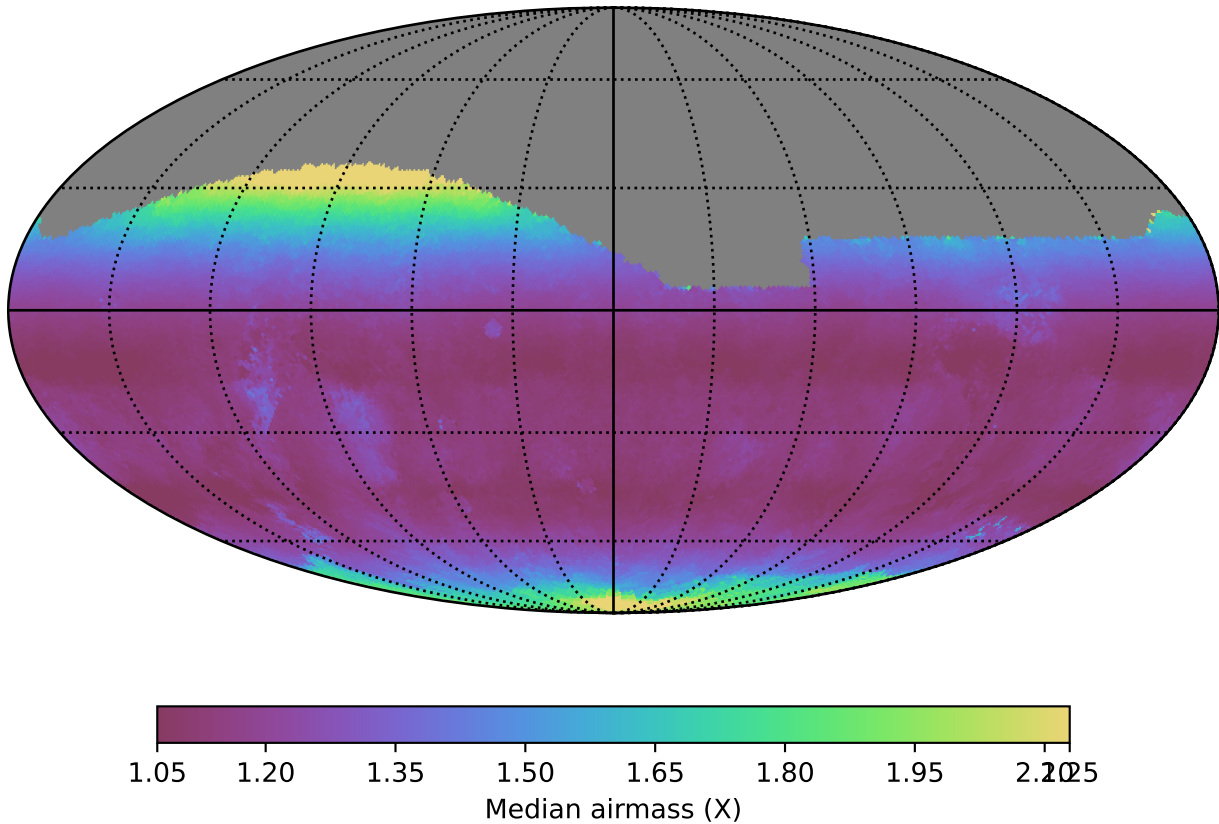
early_u_fpextra2.0_v3.4_10yrs All sky g band: Median airmass
