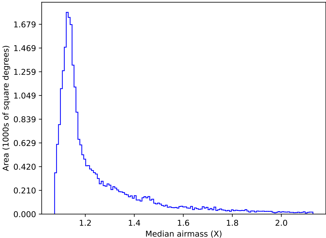
early_u_fpextra2.0_v3.4_10yrs All sky g band: Median airmass
