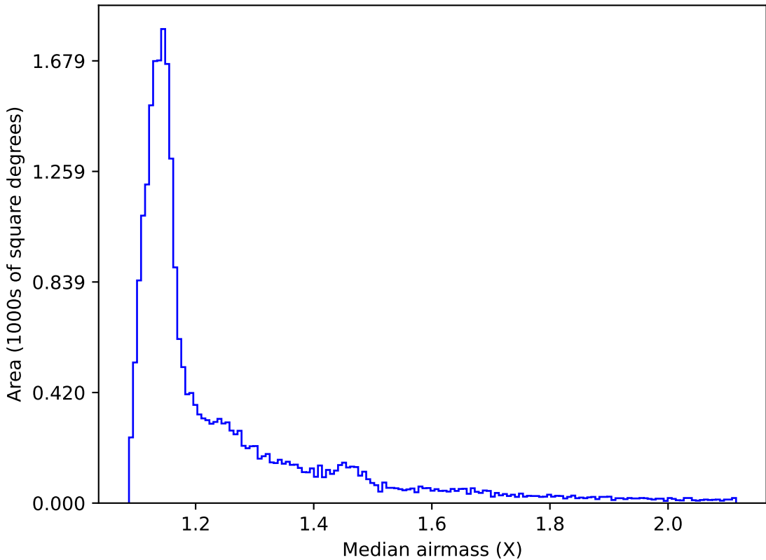
early_u_fpextra2.0_v3.4_10yrs All sky all bands: Median airmass
