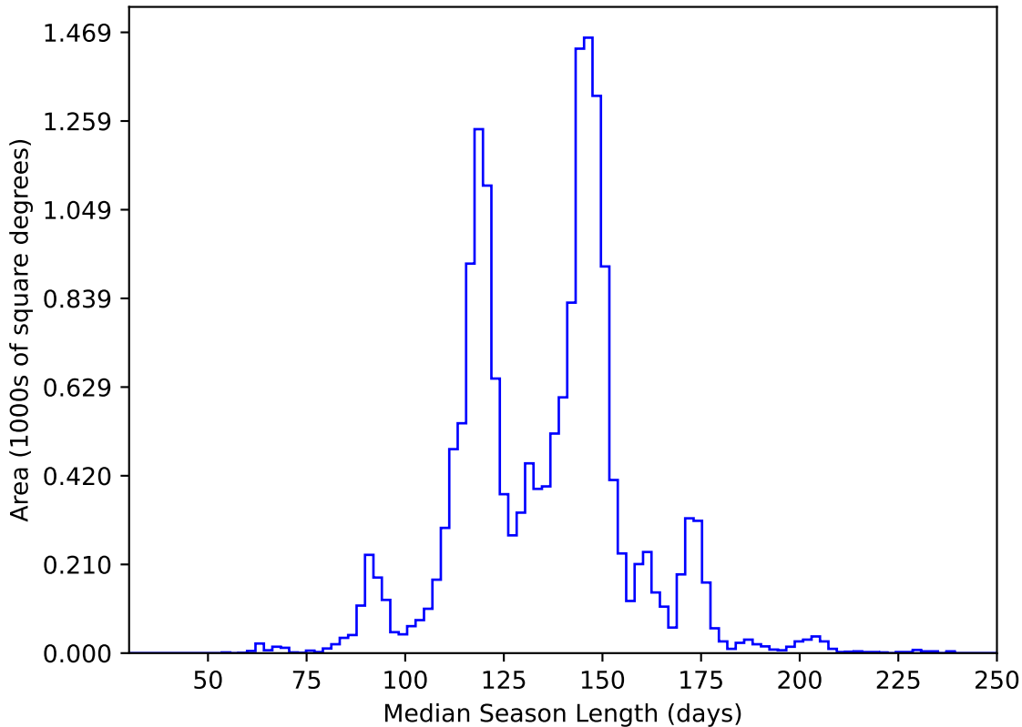
early_u_fpextra2.0_v3.4_10yrs WFD y band: Median Season Length
