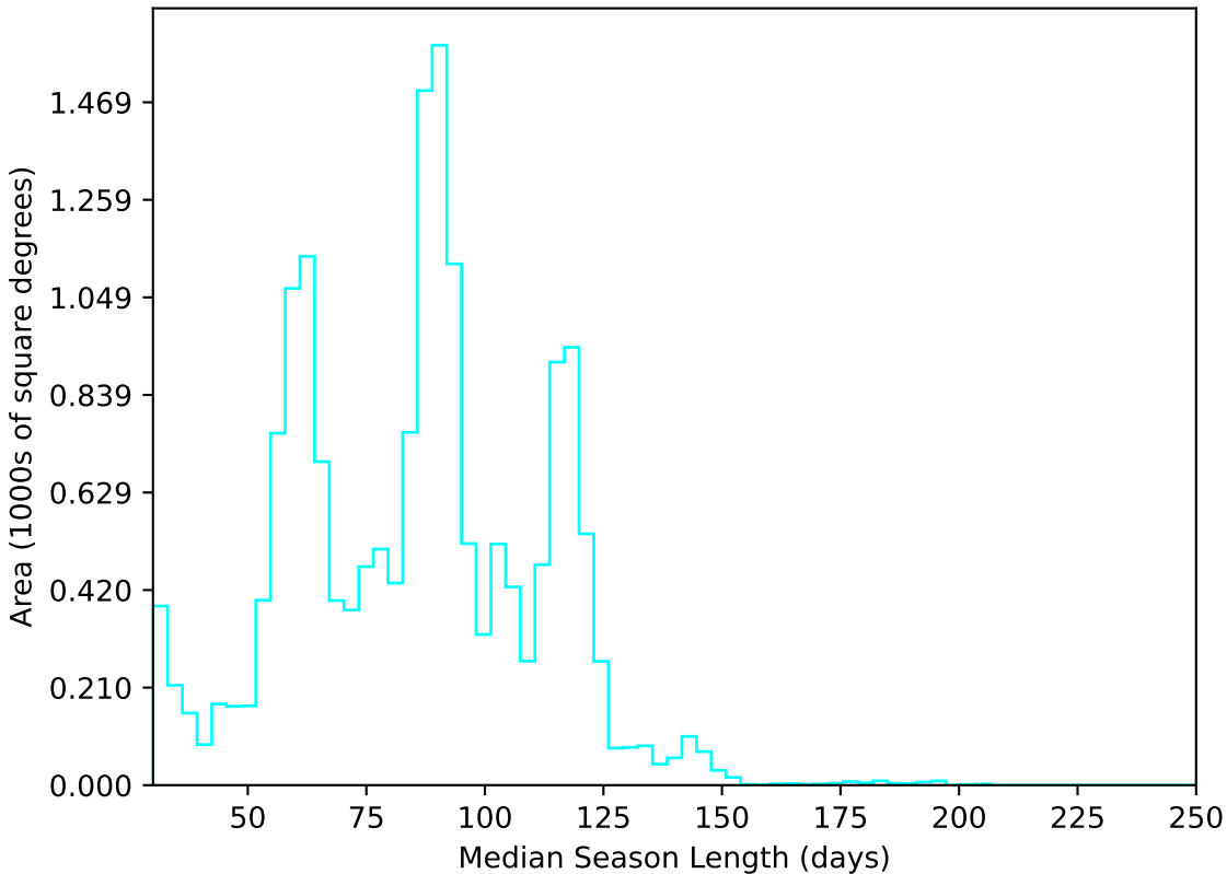
early_u_fpextra2.0_v3.4_10yrs WFD u band: Median Season Length
