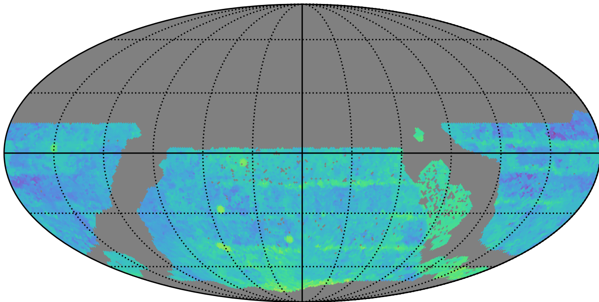
early_u_fpextra2.0_v3.4_10yrs WFD r band: Median Season Length
