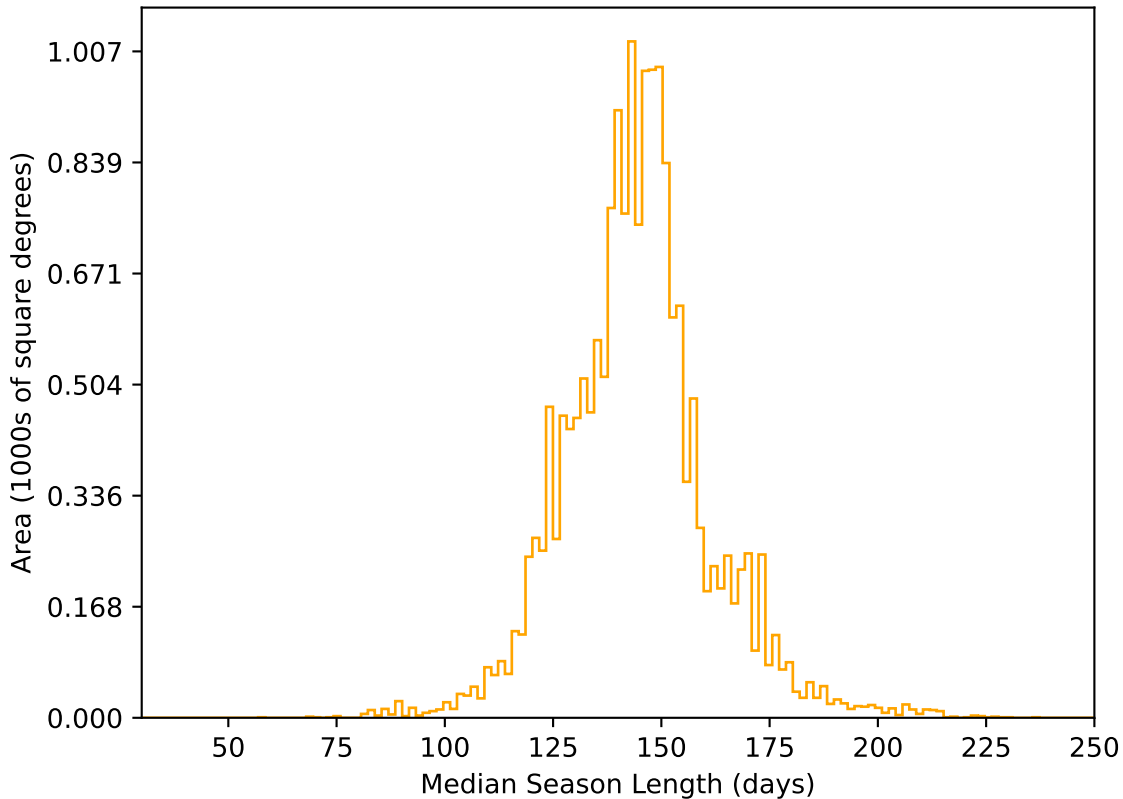
early_u_fpextra2.0_v3.4_10yrs WFD r band: Median Season Length
