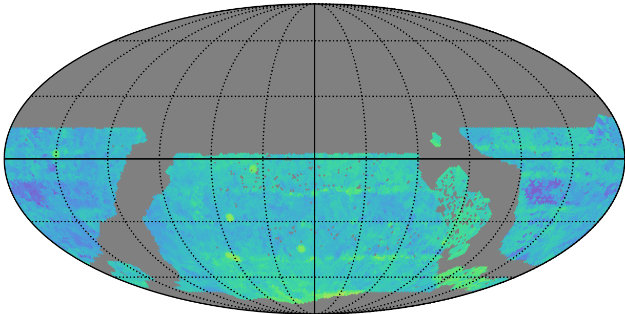
early_u_fpextra2.0_v3.4_10yrs WFD i band: Median Season Length
