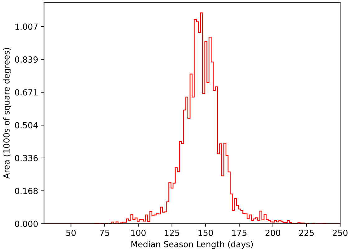
early_u_fpextra2.0_v3.4_10yrs WFD i band: Median Season Length
