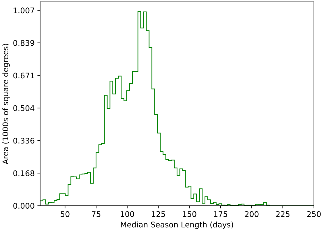
early_u_fpextra2.0_v3.4_10yrs WFD g band: Median Season Length
