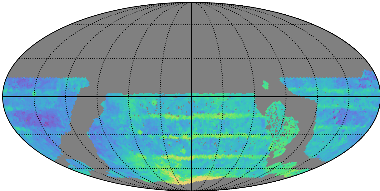
early_u_fpextra2.0_v3.4_10yrs WFD all bands: Median Season Length
