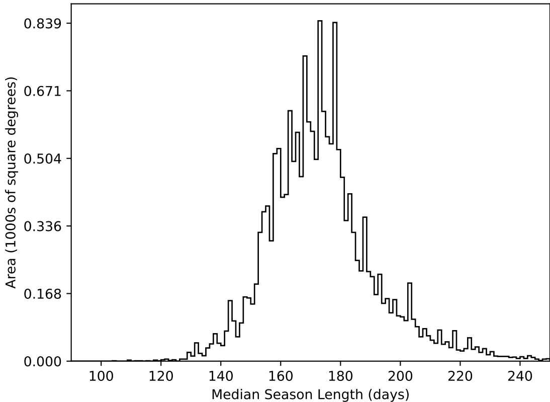
early_u_fpextra2.0_v3.4_10yrs WFD all bands: Median Season Length
