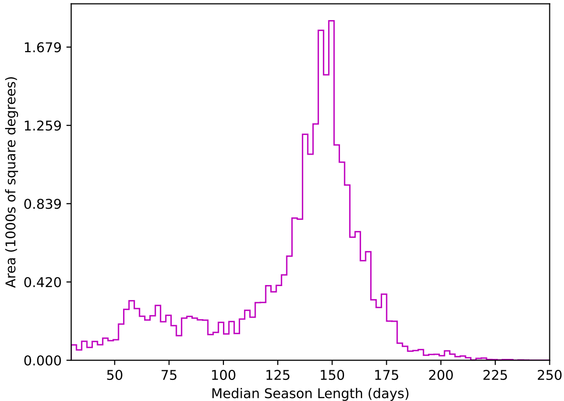
early_u_fpextra2.0_v3.4_10yrs All sky z band: Median Season Length
