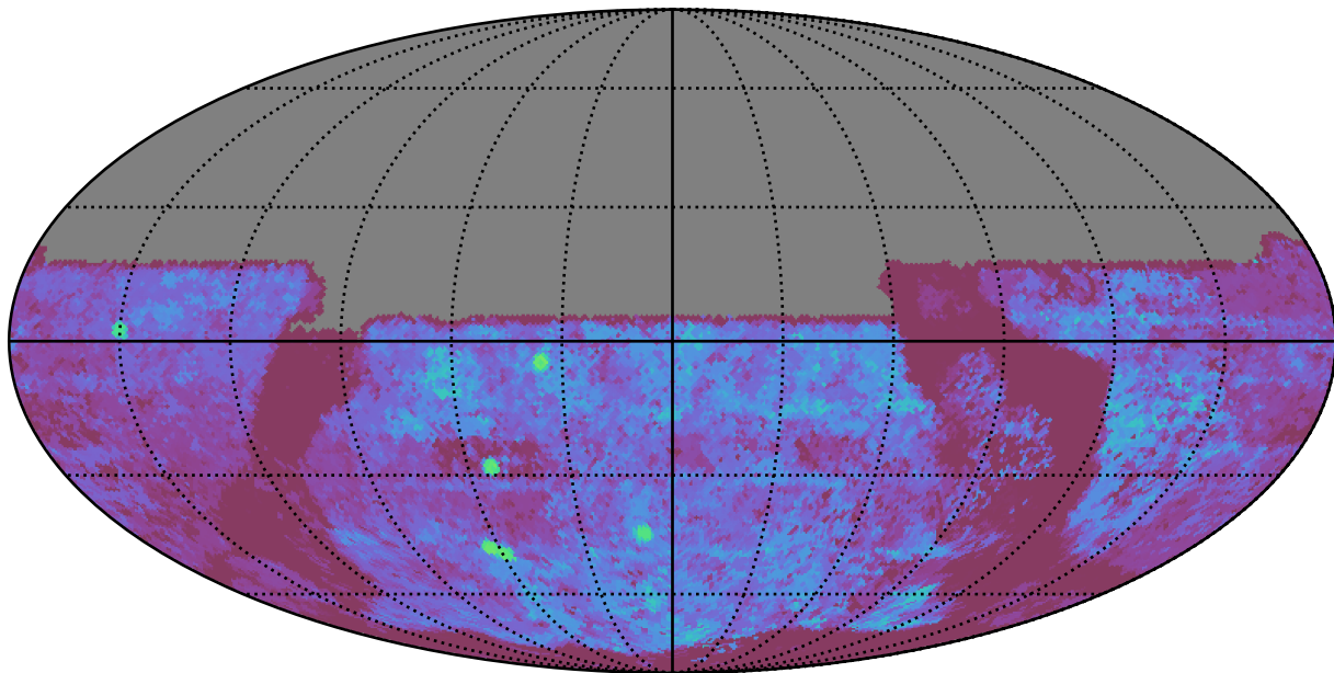
early_u_fpextra2.0_v3.4_10yrs All sky u band: Median Season Length
