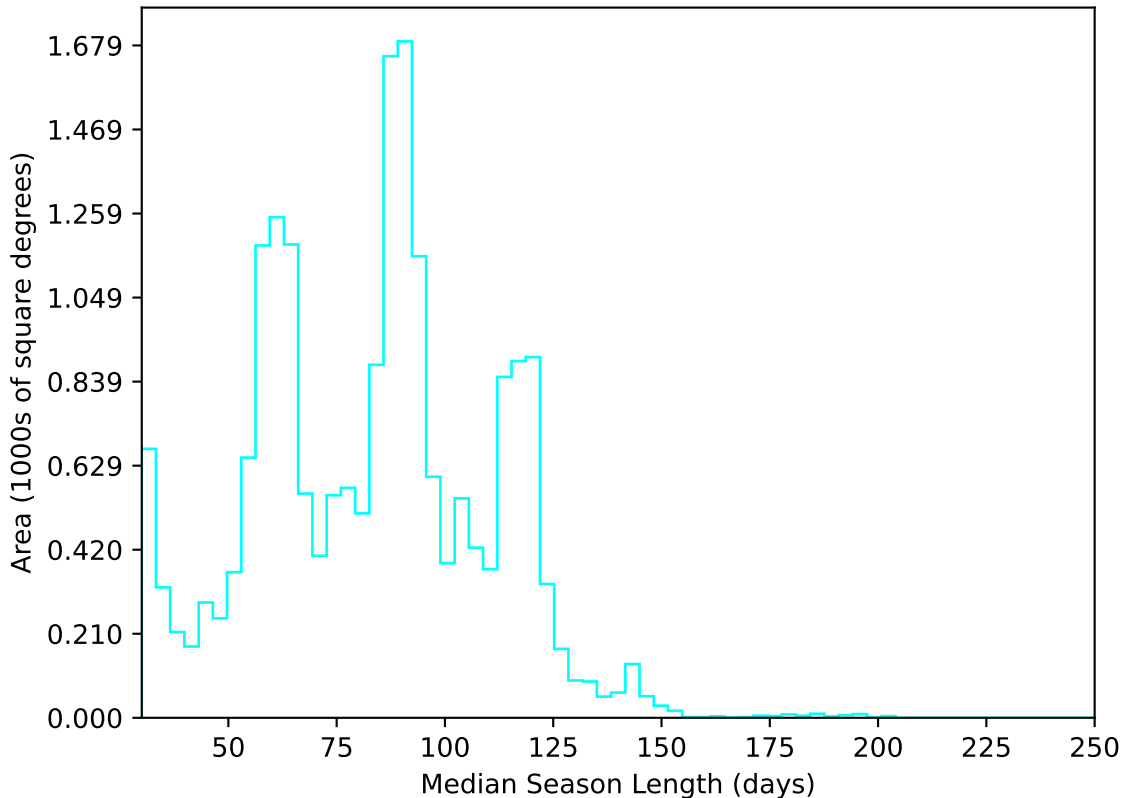
early_u_fpextra2.0_v3.4_10yrs All sky u band: Median Season Length
