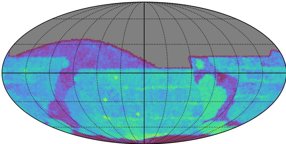
early_u_fpextra2.0_v3.4_10yrs All sky r band: Median Season Length
