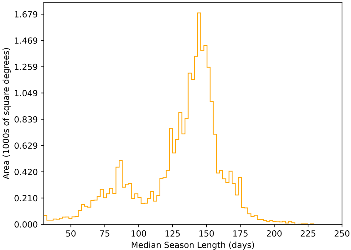
early_u_fpextra2.0_v3.4_10yrs All sky r band: Median Season Length
