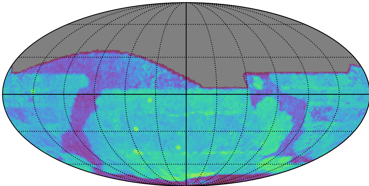
early_u_fpextra2.0_v3.4_10yrs All sky i band: Median Season Length
