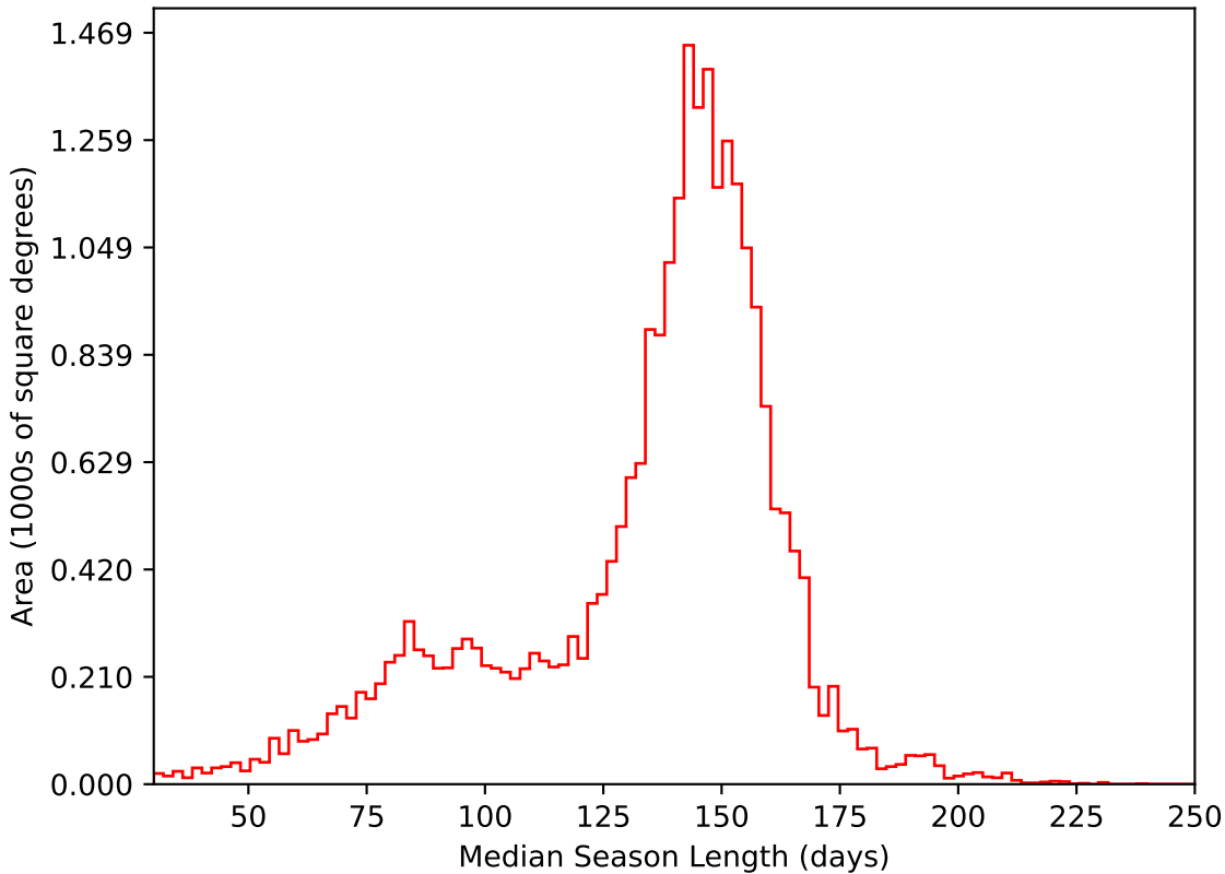
early_u_fpextra2.0_v3.4_10yrs All sky i band: Median Season Length
