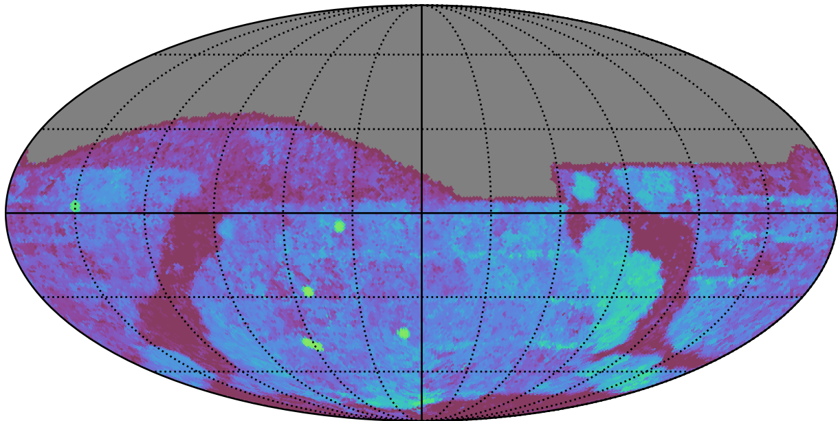
early_u_fpextra2.0_v3.4_10yrs All sky g band: Median Season Length
