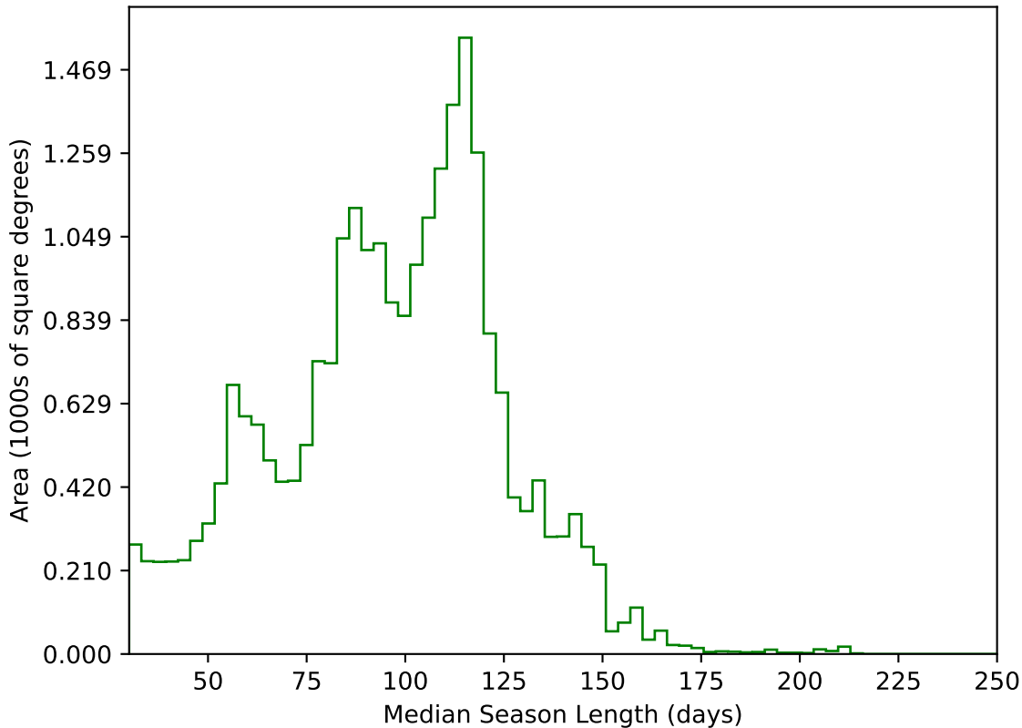
early_u_fpextra2.0_v3.4_10yrs All sky g band: Median Season Length
