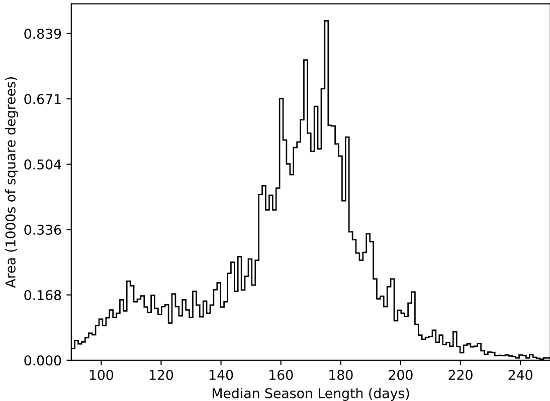
early_u_fpextra2.0_v3.4_10yrs All sky all bands: Median Season Length
