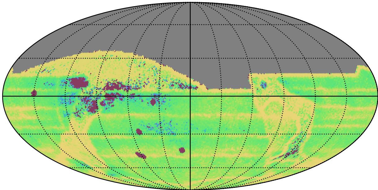
early_u_fpextra2.0_v3.4_10yrs All sky: Median Intra-Night Gap
