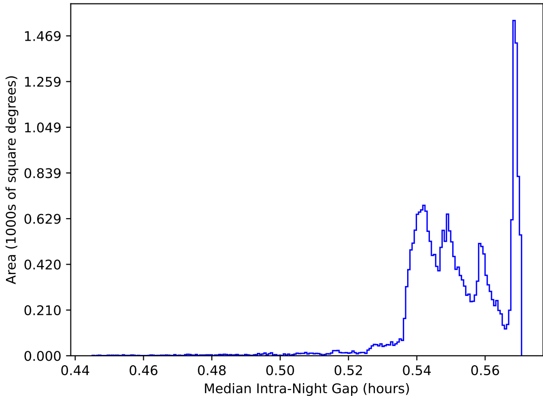
early_u_fpextra2.0_v3.4_10yrs All sky: Median Intra-Night Gap
