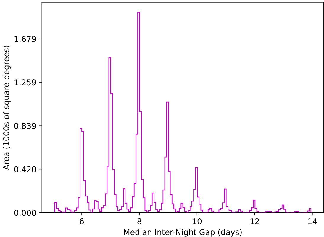
early_u_fpextra2.0_v3.4_10yrs WFD z band: Median Inter-Night Gap
