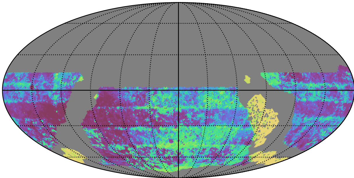
early_u_fpextra2.0_v3.4_10yrs WFD y band: Median Inter-Night Gap
