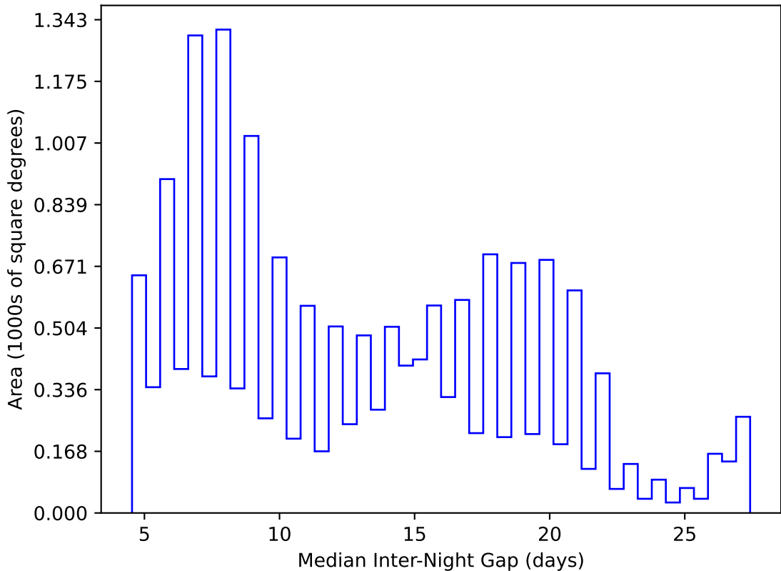
early_u_fpextra2.0_v3.4_10yrs WFD y band: Median Inter-Night Gap
