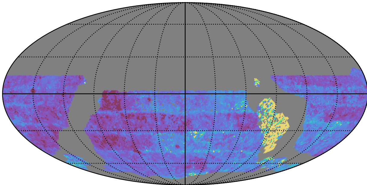
early_u_fpextra2.0_v3.4_10yrs WFD u band: Median Inter-Night Gap
