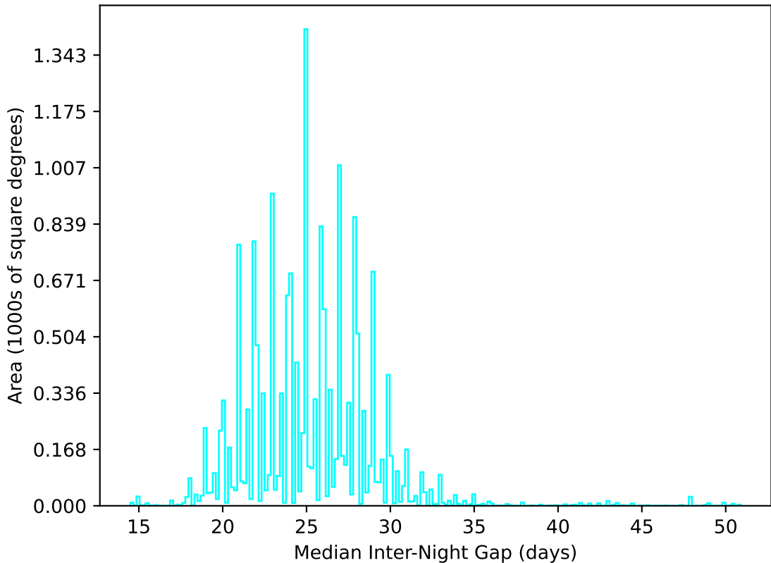
early_u_fpextra2.0_v3.4_10yrs WFD u band: Median Inter-Night Gap
