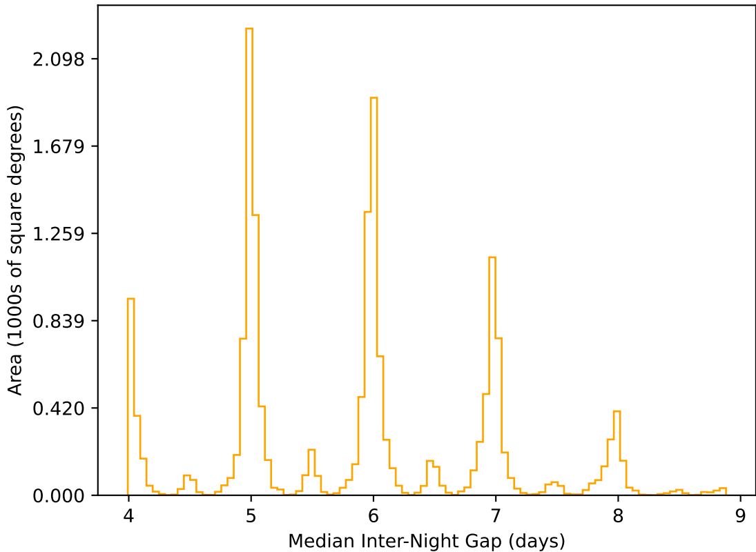
early_u_fpextra2.0_v3.4_10yrs WFD r band: Median Inter-Night Gap
