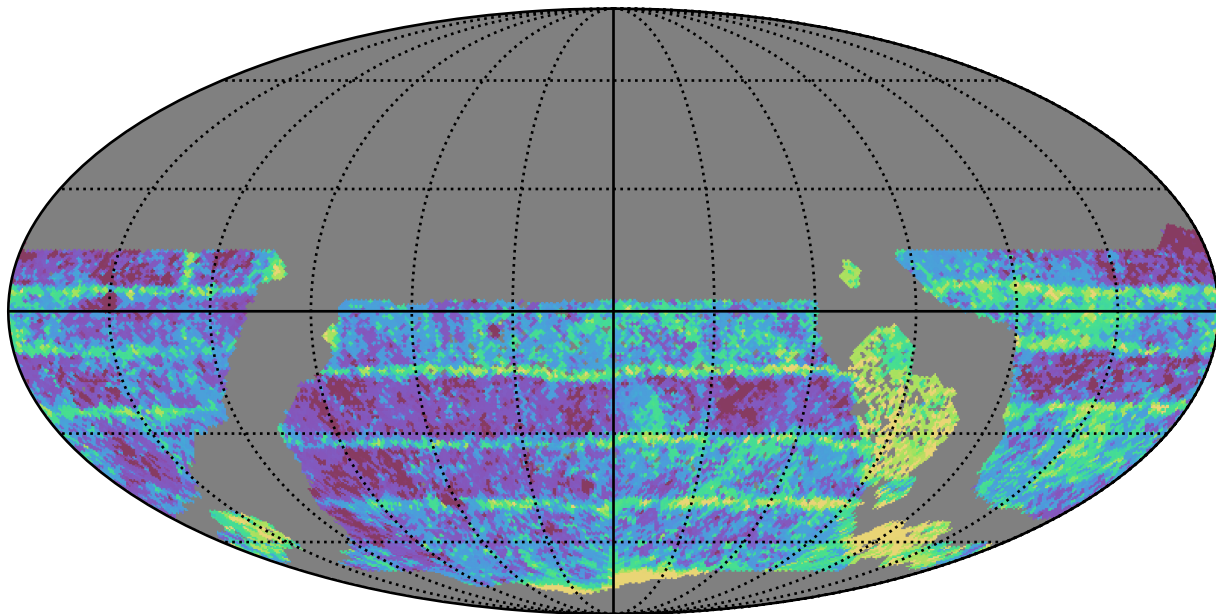
early_u_fpextra2.0_v3.4_10yrs WFD i band: Median Inter-Night Gap
