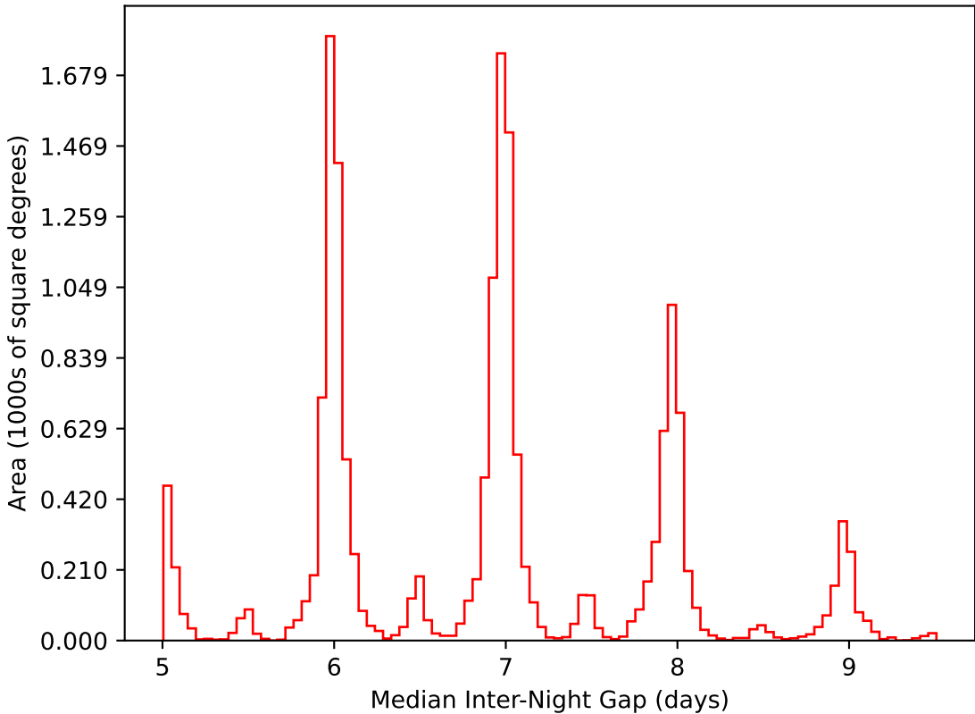
early_u_fpextra2.0_v3.4_10yrs WFD i band: Median Inter-Night Gap
