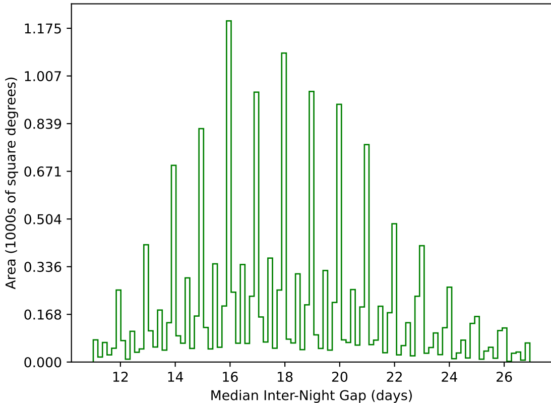
early_u_fpextra2.0_v3.4_10yrs WFD g band: Median Inter-Night Gap
