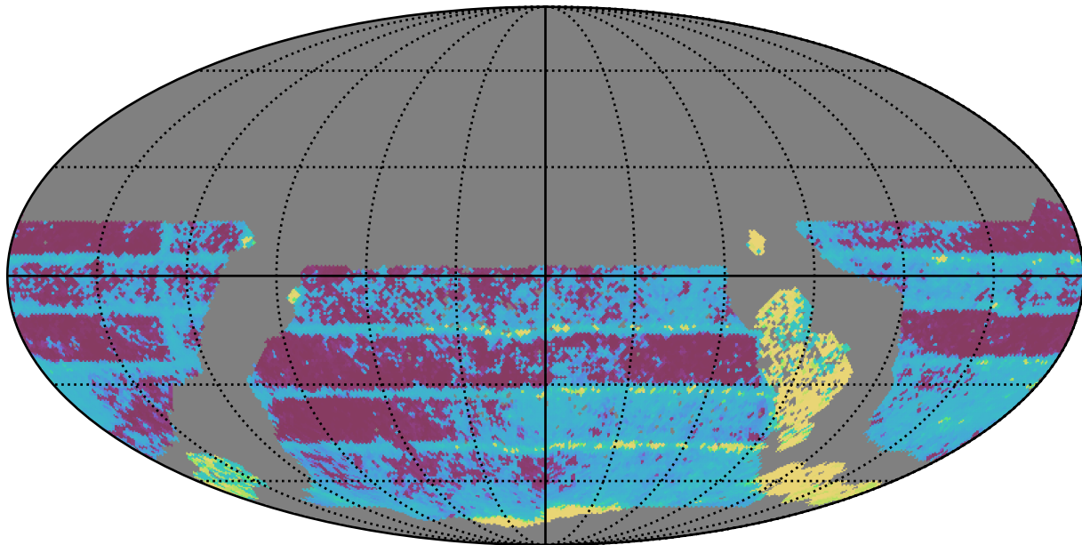
early_u_fpextra2.0_v3.4_10yrs WFD all bands: Median Inter-Night Gap
