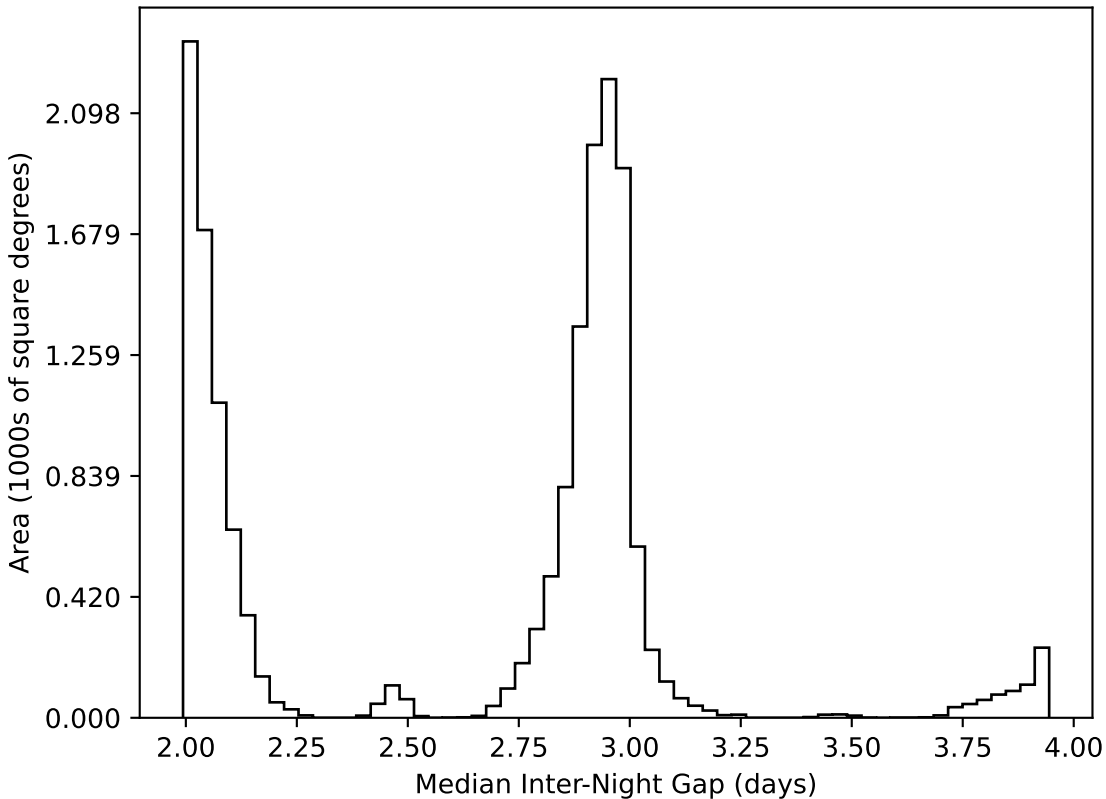
early_u_fpextra2.0_v3.4_10yrs WFD all bands: Median Inter-Night Gap
