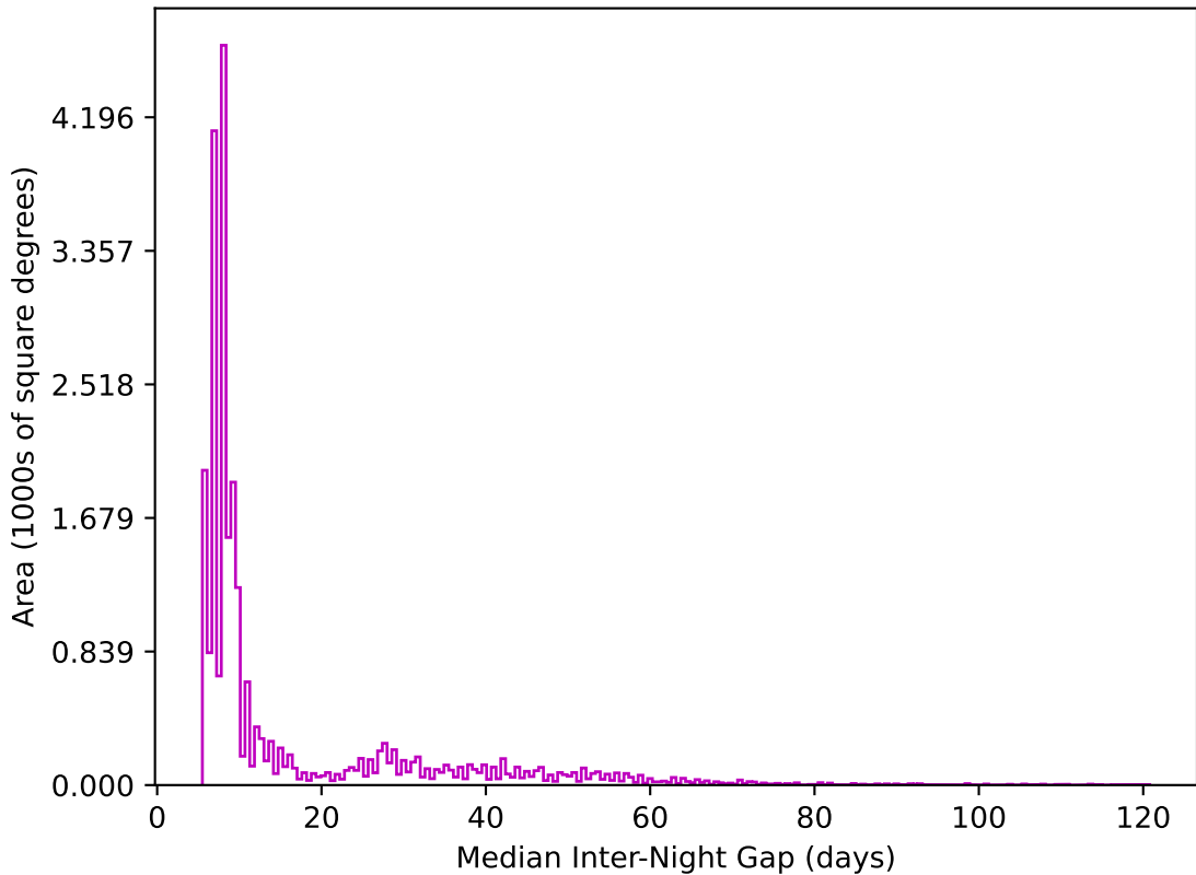
early_u_fpextra2.0_v3.4_10yrs All sky z band: Median Inter-Night Gap
