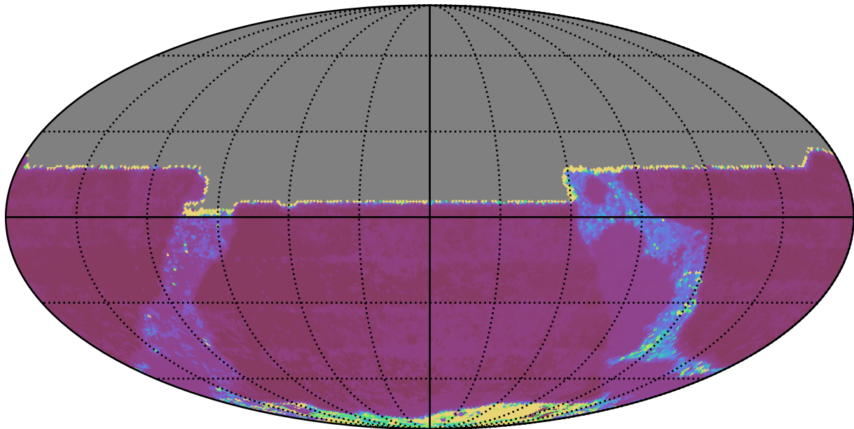
early_u_fpextra2.0_v3.4_10yrs All sky y band: Median Inter-Night Gap
