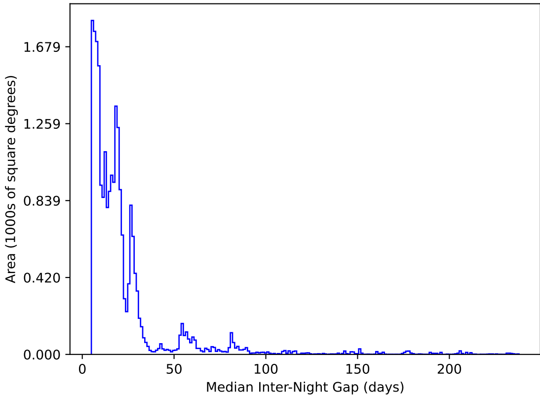
early_u_fpextra2.0_v3.4_10yrs All sky y band: Median Inter-Night Gap
