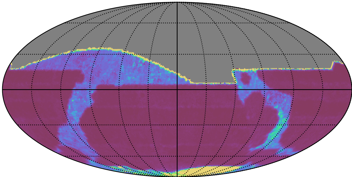
early_u_fpextra2.0_v3.4_10yrs All sky r band: Median Inter-Night Gap
