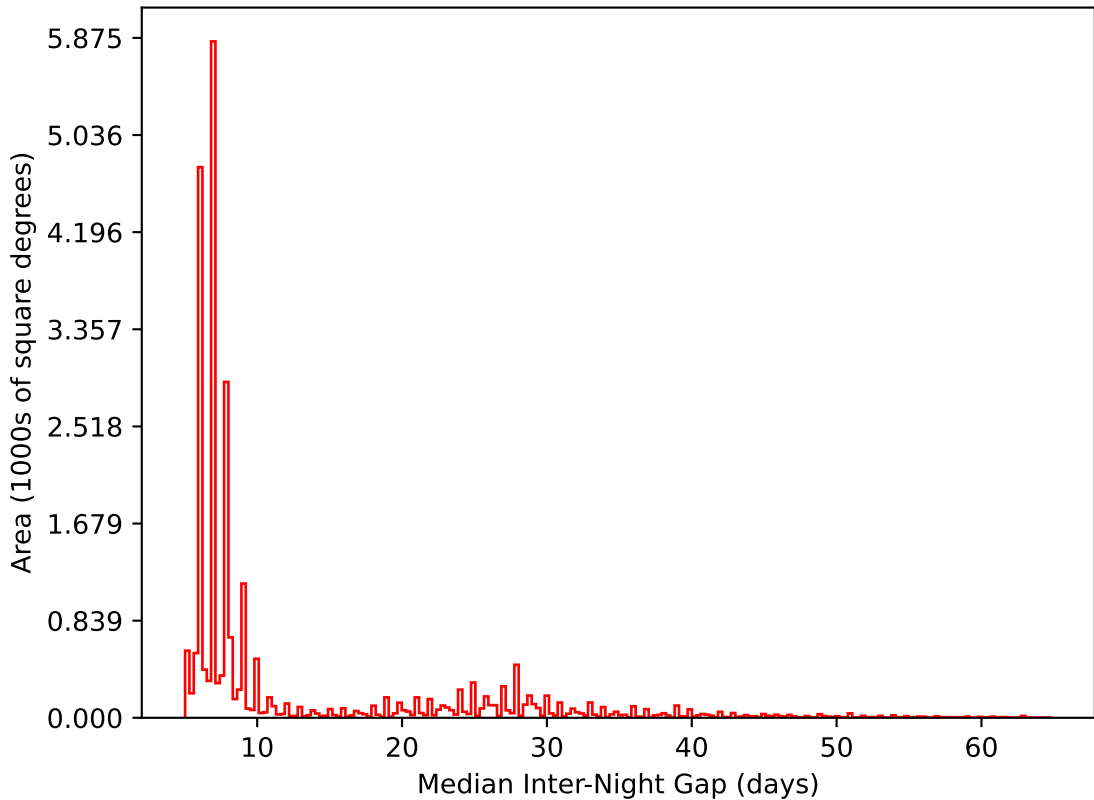
early_u_fpextra2.0_v3.4_10yrs All sky i band: Median Inter-Night Gap
