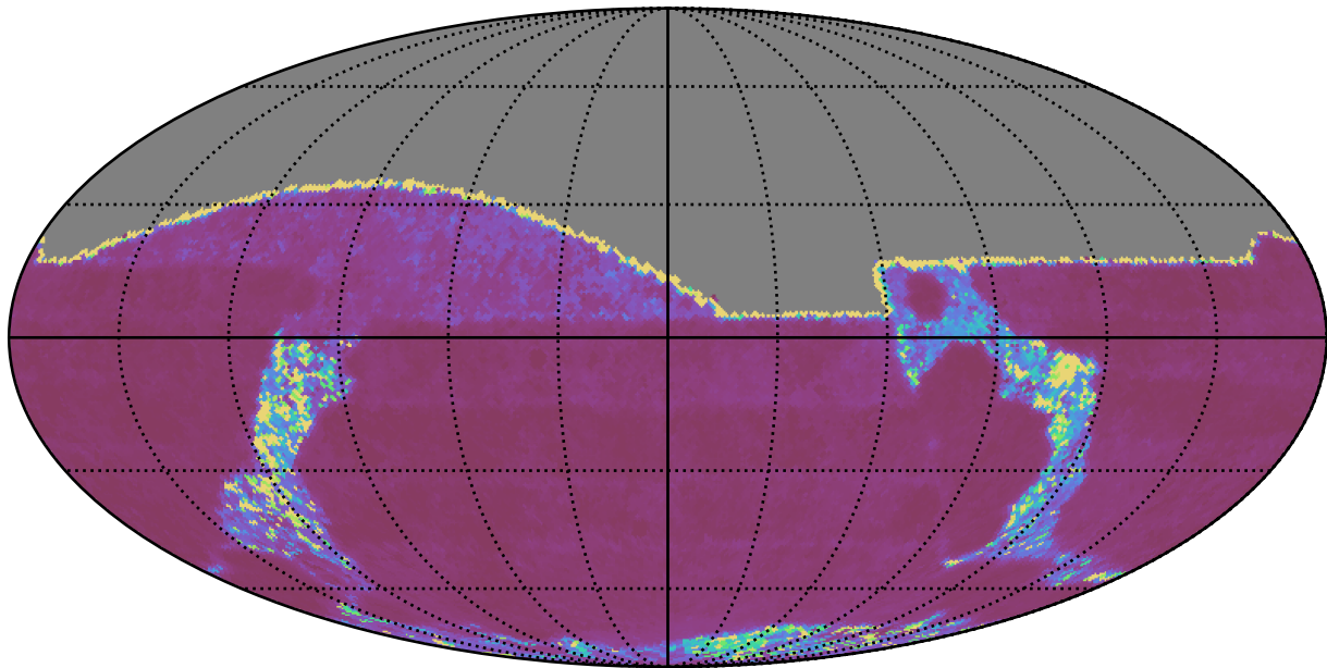
early_u_fpextra2.0_v3.4_10yrs All sky g band: Median Inter-Night Gap
