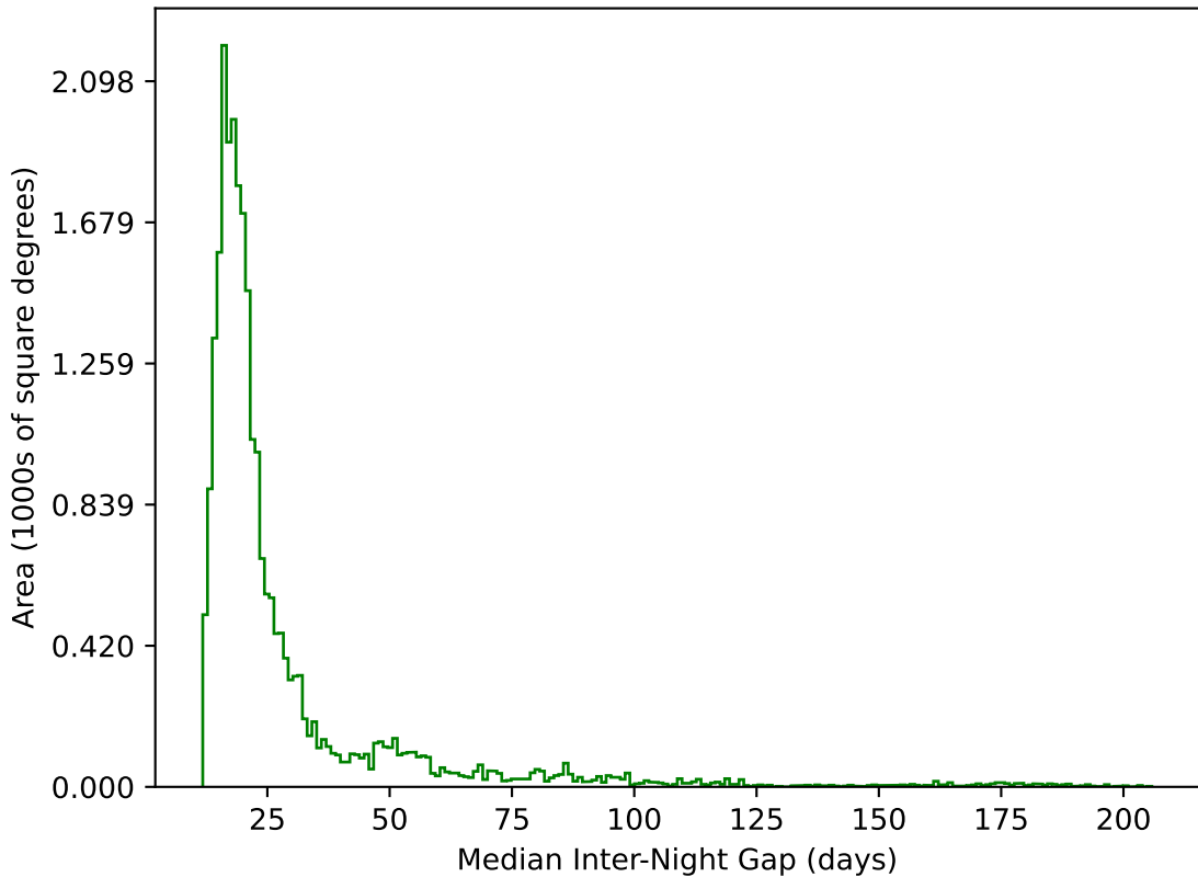
early_u_fpextra2.0_v3.4_10yrs All sky g band: Median Inter-Night Gap
