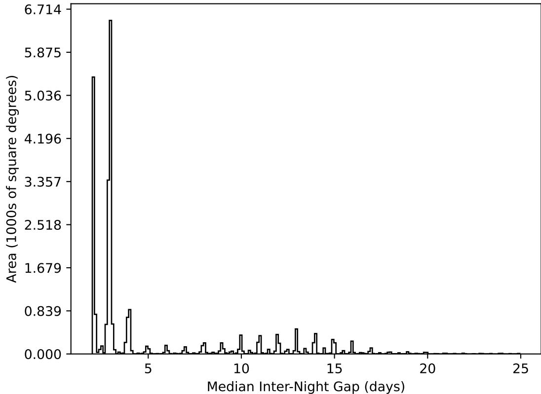
early_u_fpextra2.0_v3.4_10yrs All sky all bands: Median Inter-Night Gap
