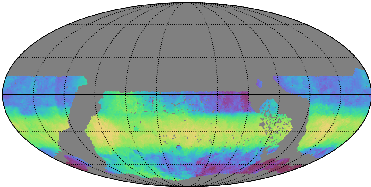
early_u_fpextra2.0_v3.4_10yrs WFD z band: Median HA
