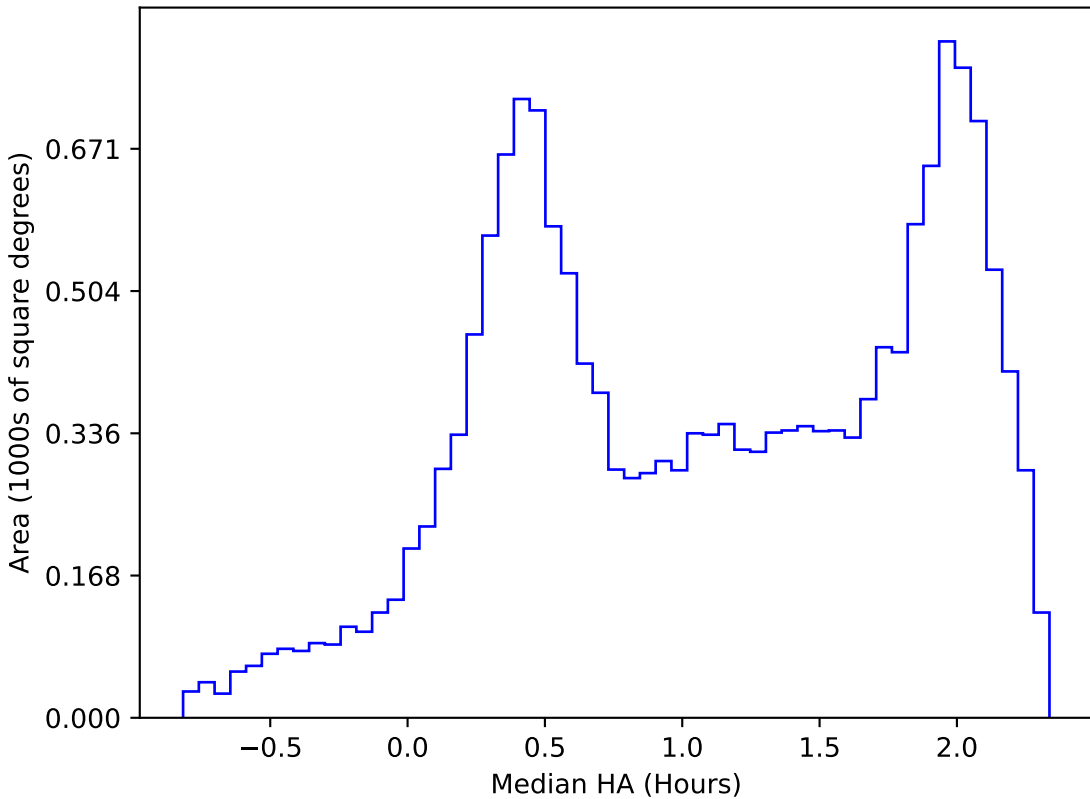
early_u_fpextra2.0_v3.4_10yrs WFD z band: Median HA
