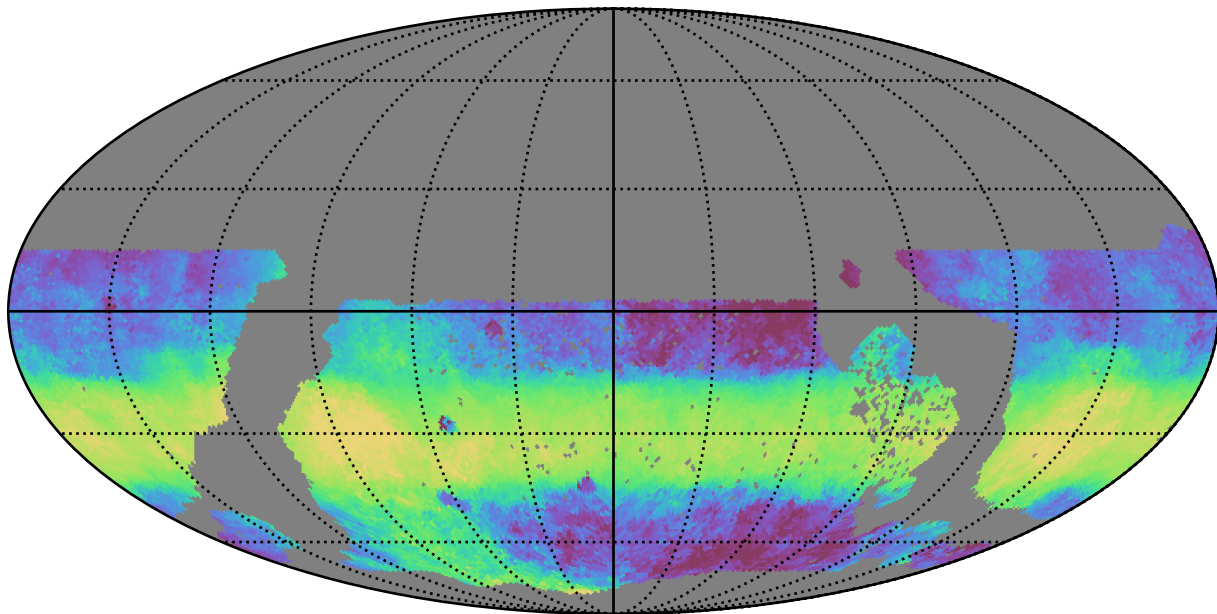
early_u_fpextra2.0_v3.4_10yrs WFD y band: Median HA
