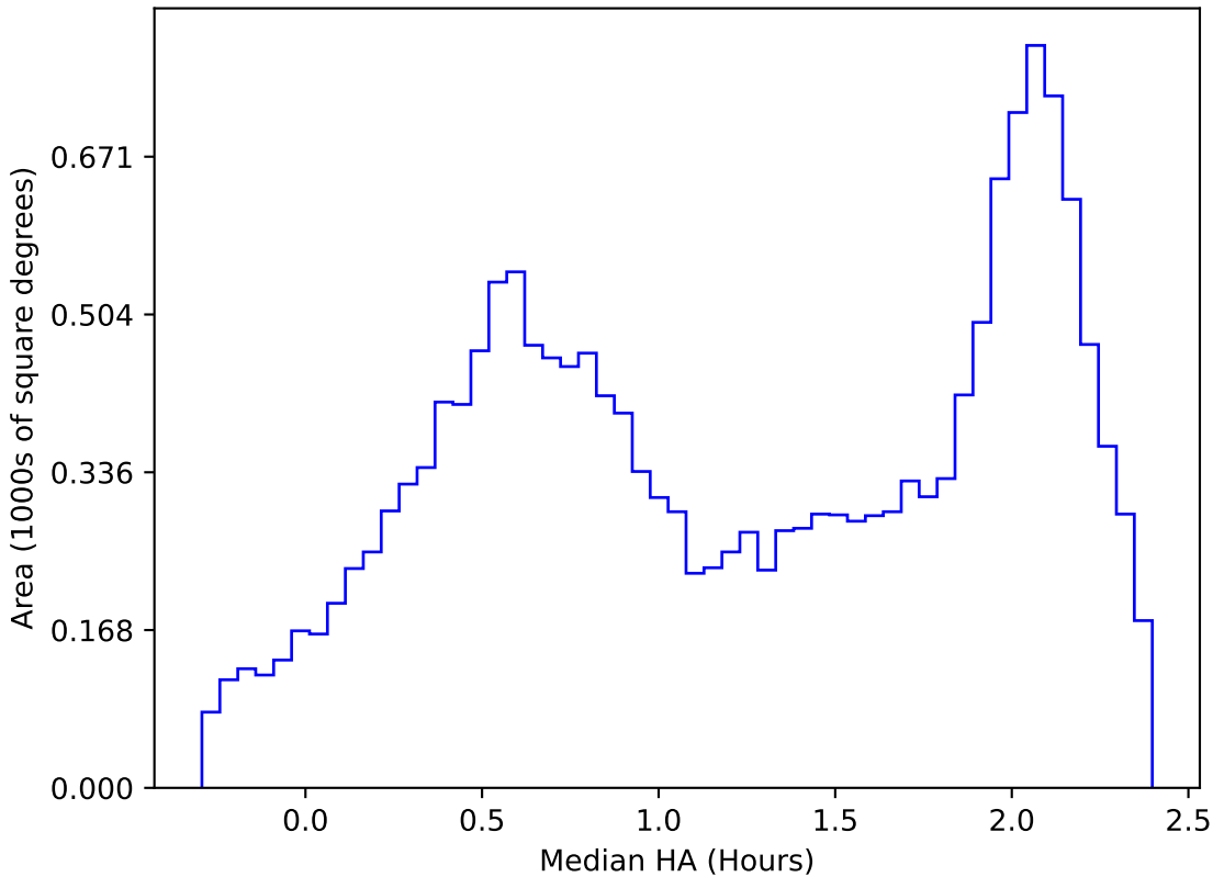
early_u_fpextra2.0_v3.4_10yrs WFD y band: Median HA
