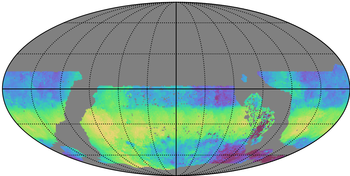
early_u_fpextra2.0_v3.4_10yrs WFD u band: Median HA
