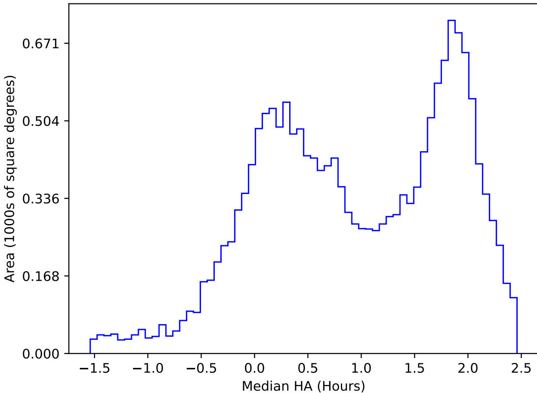
early_u_fpextra2.0_v3.4_10yrs WFD u band: Median HA
