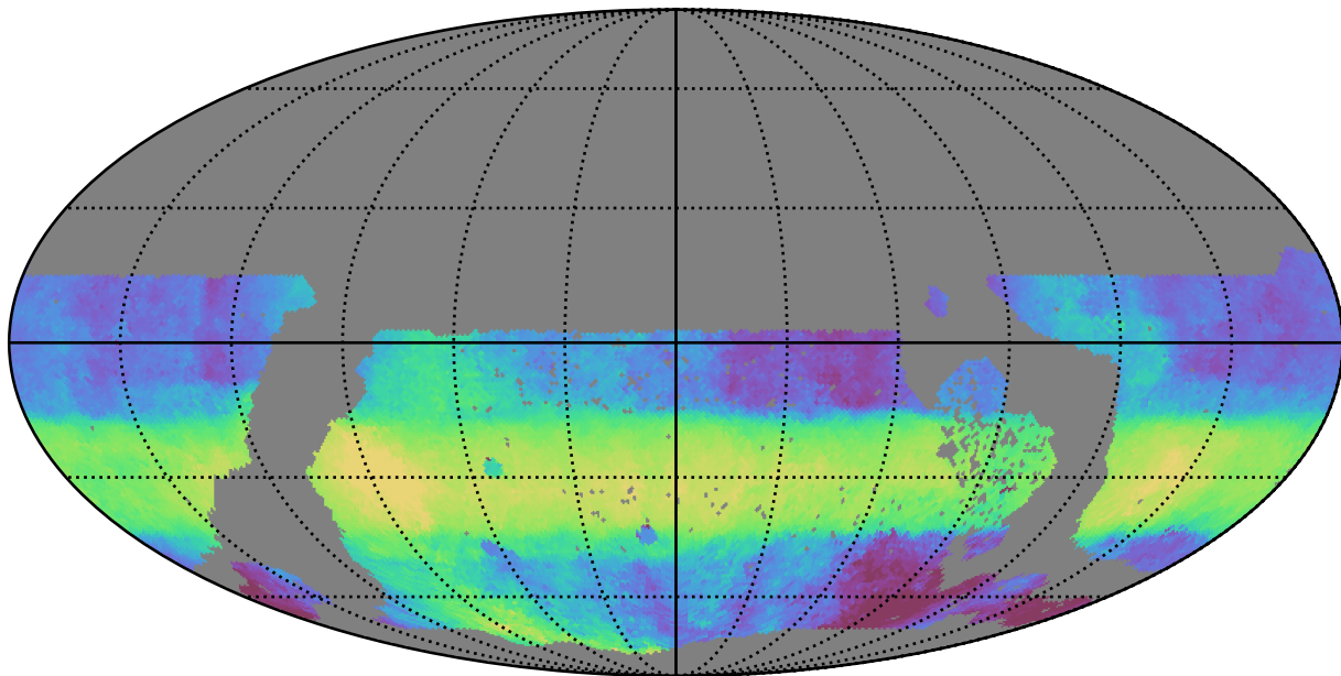
early_u_fpextra2.0_v3.4_10yrs WFD r band: Median HA
